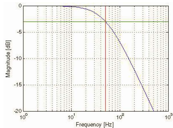
Figure 8-74 Current Actual Value Averaged – Amplitude Response
