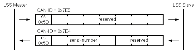
Figure 7-70 LSS – Inquire Identity Serial Number
