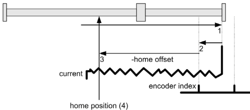
Figure 5-18 Homing Method -1
