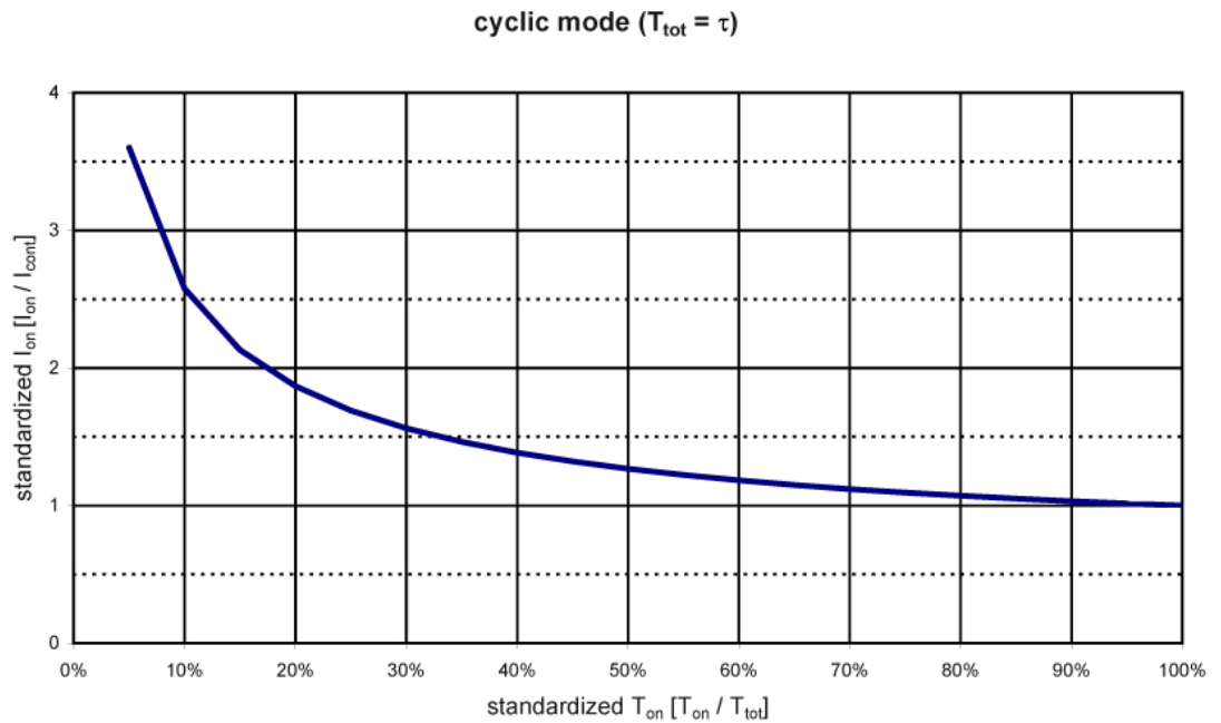
Figure 5-41 Cyclic Mode standardized I_{\text{on}} vs. Standardized T_{\text{on}}
