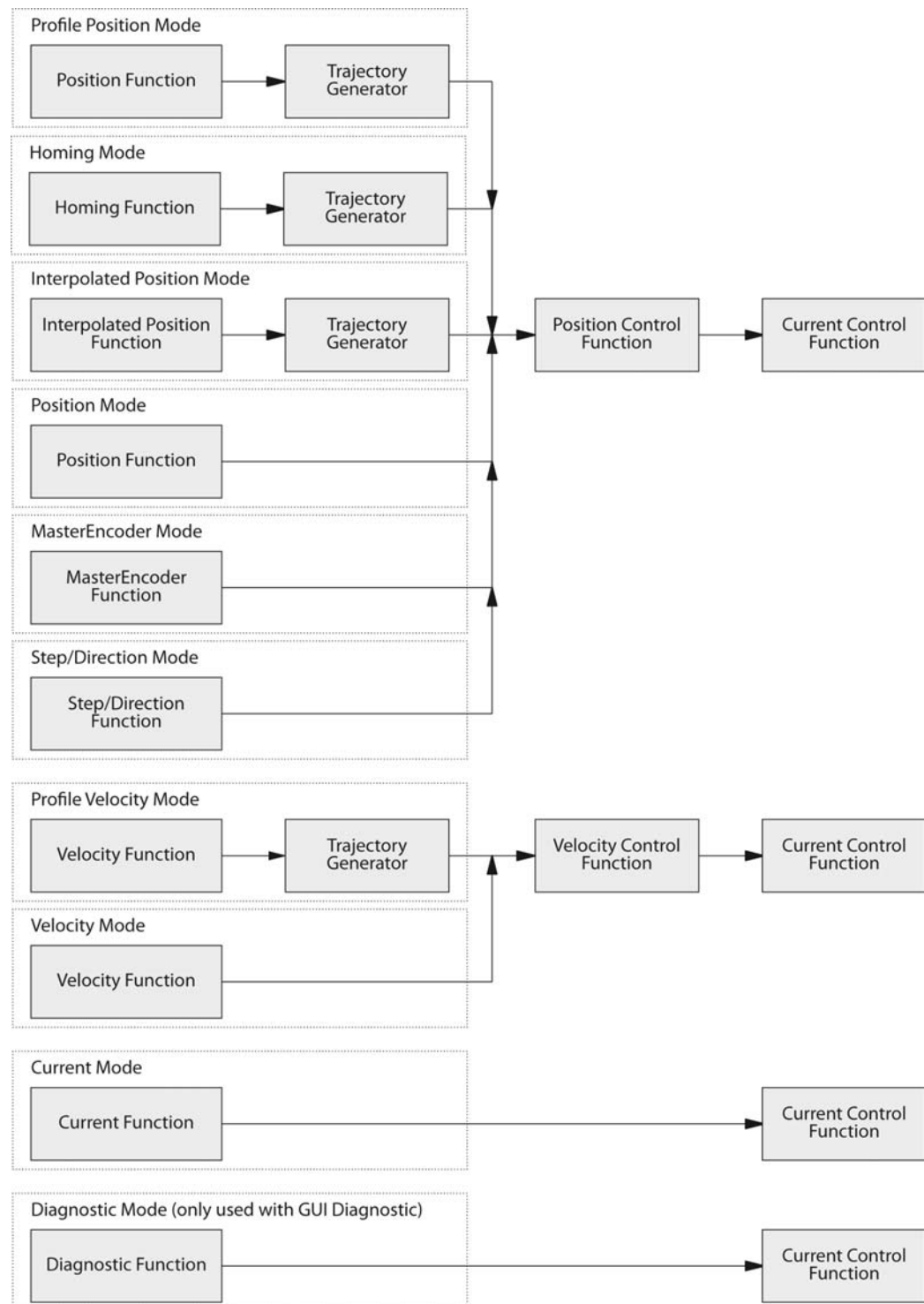
Figure 5-4 Functional Architecture
