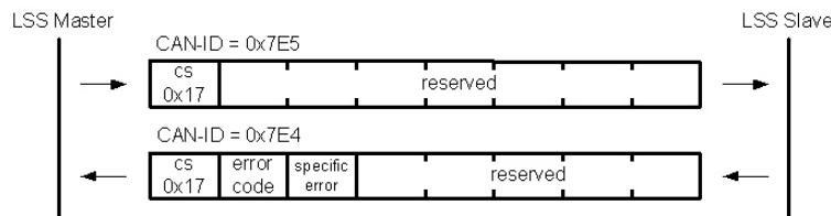
Figure 7-66 LSS – Store Configuration
