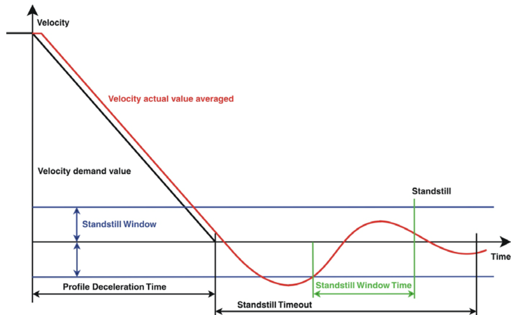
Figure 8-78 Standstill Window
