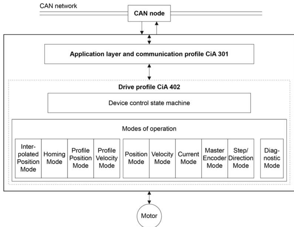
Figure 3-2 Communication Architecture
