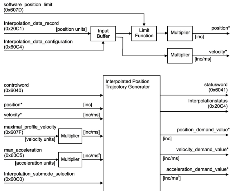
Figure 5-22 Interpolated Position Mode – Interpolation Controller
