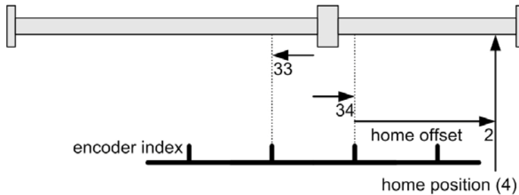
Figure 5-17 Homing Methods 33 and 34
