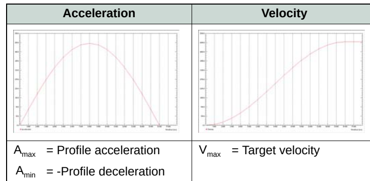
Figure 5-35 Profile Velocity Trajectory – Sin² Ramp (sinusoidal Profile)
