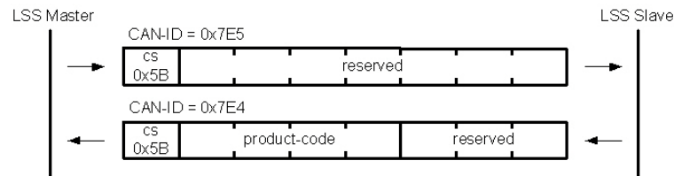
Figure 7-68 LSS – Inquire Identity Product Code
